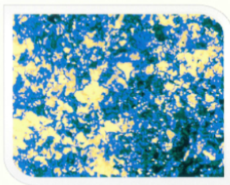
Microstructure of Alloy cast steel roll, 35/40 ShC having pearlitic matrix and carbides. Magnification : 500X
